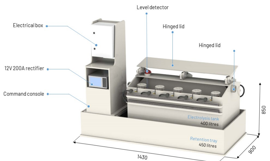
Fig.2 Electrolysis system
